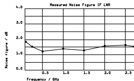
Fig. 9: Measured IF LNA noise figure
