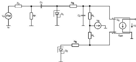
Fig. 17: Detector circuit schematic
