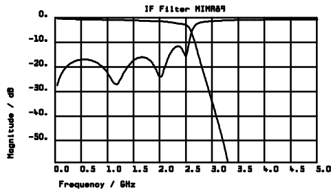
Fig. 16: Measured response of the IF filter
