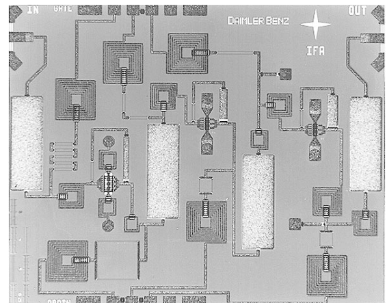
Fig.10: Photograph of the IF LNA chip
