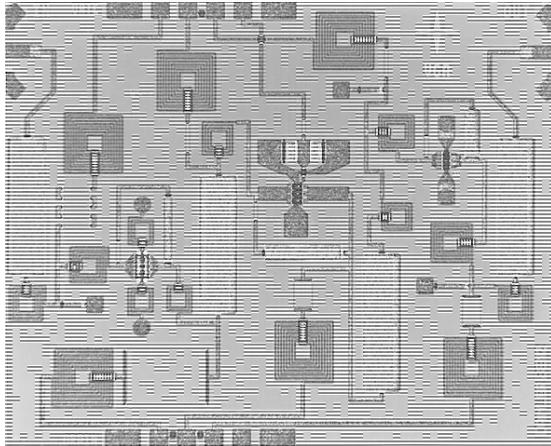
Fig. 12: Photograph of the VGA chip
