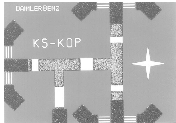
Fig. 8: IF coupler chip
