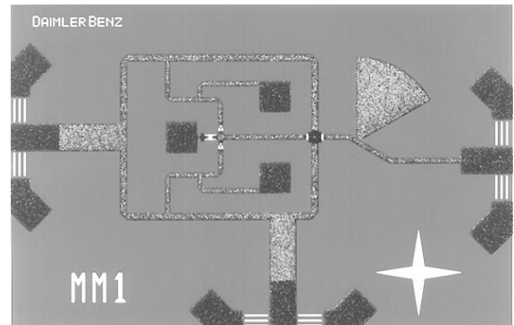
Fig.2: DSB mixer chip
