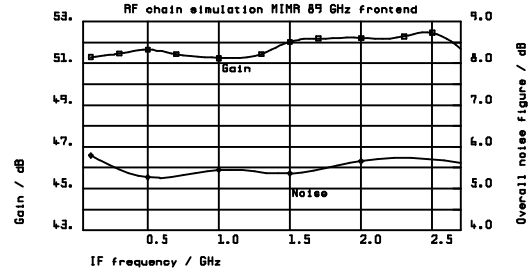
Fig. 18: Simulation of the radiometer RF chain
