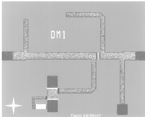
Fig. 6: Doubler chip 44.5 GHz
