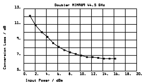
Fig. 7: Conversion loss of the 44.5 GHz doubler
