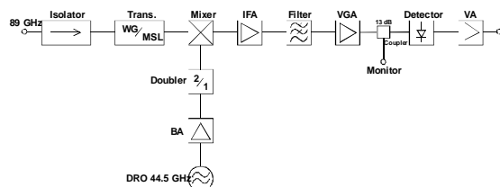
Fig. 1: Block diagram of the MIMR 89 GHz frontend
