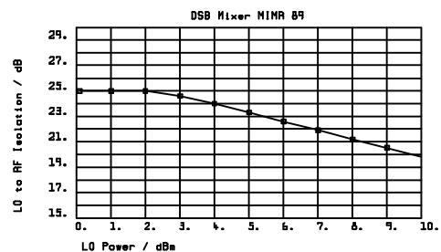
Fig.4: Mixer LO to RF isolation
